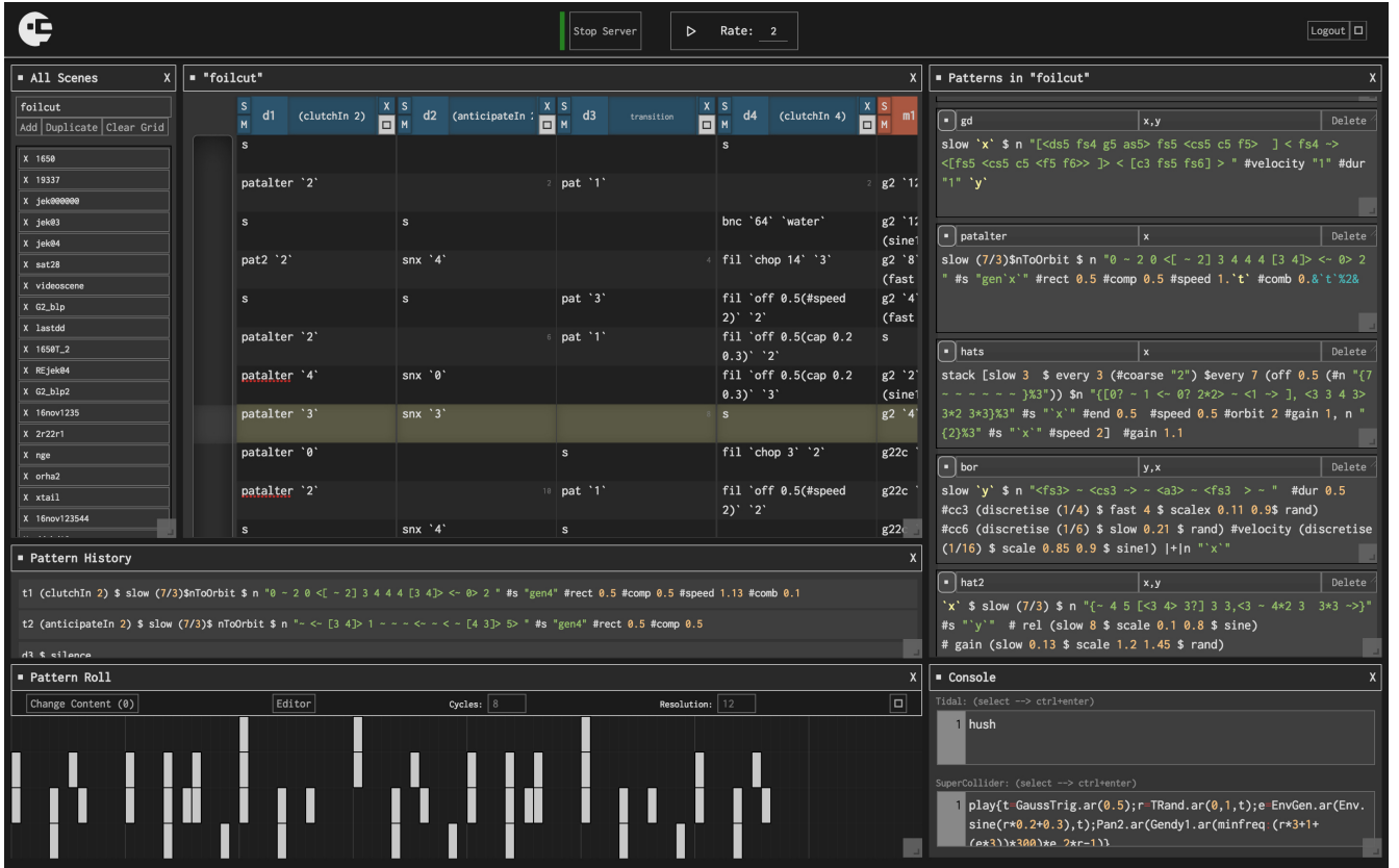
Figure 1: The user-interface – (top-left) the list of scenes; (middle) the multi-channel sequencer; (top-right) pattern dictionary; (middle-left) pattern history per channel; (bottom-left) pattern roll; (bottom-right) the text-based compiler
